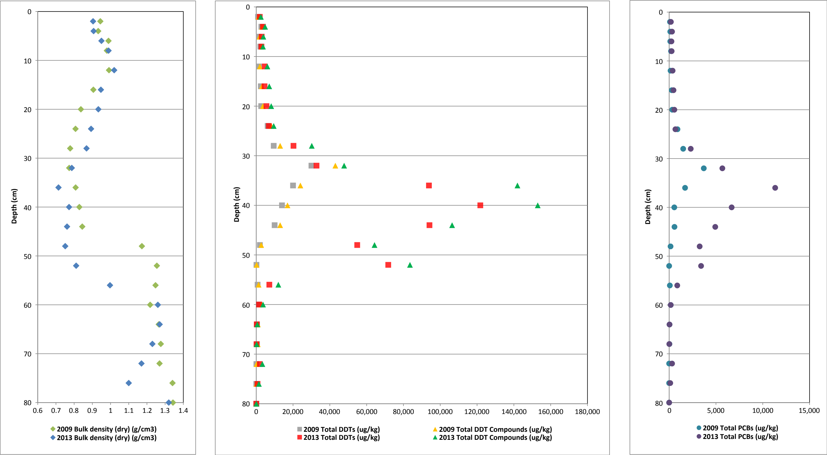
Figure 14. Vertical Profiles of Bulk Density and COCs for Core BA5C First MNR Report Palos Verdes Shelf (OU 5 of the Montrose Chemical Corp. Superfund Site) Los Angeles County, California
