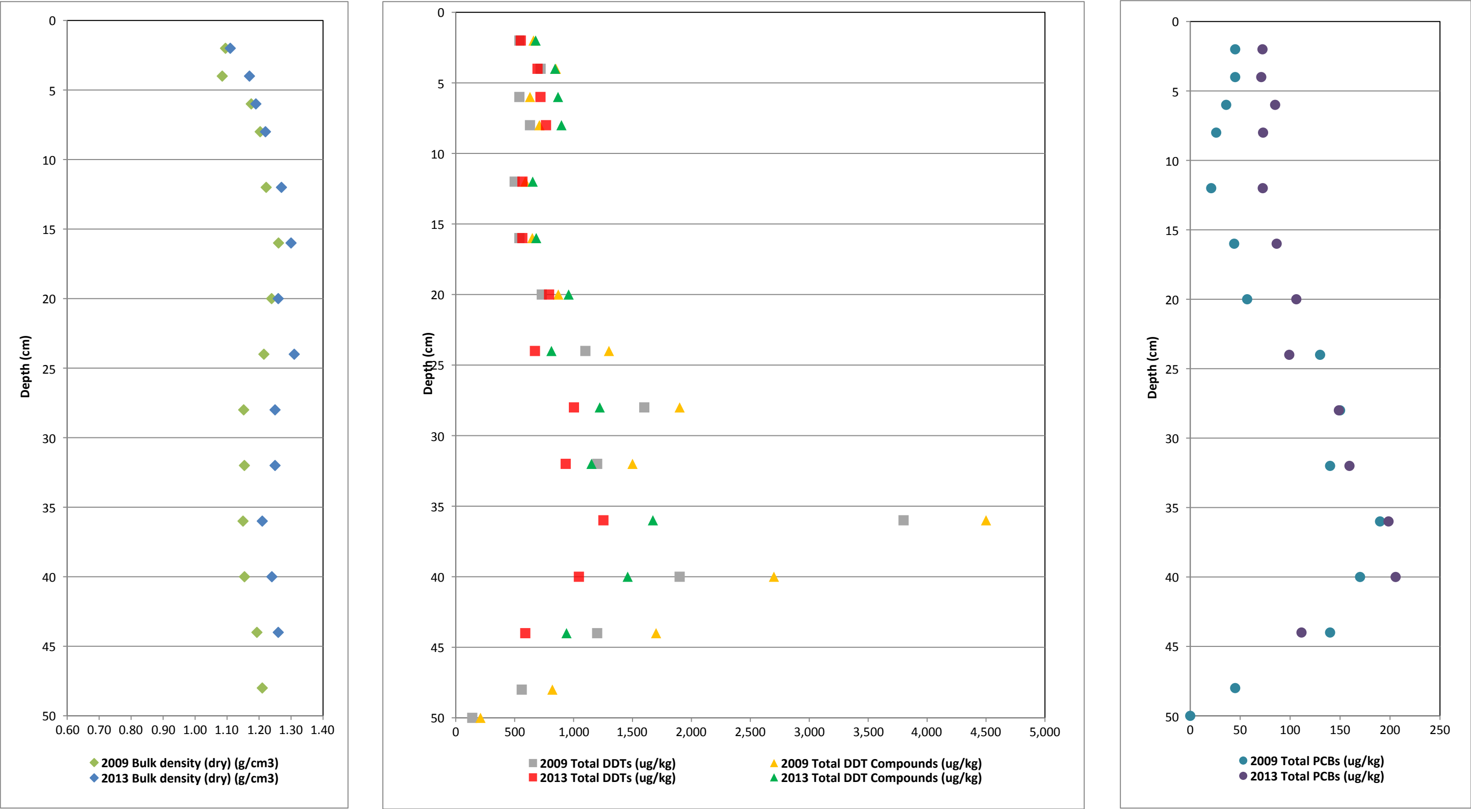
Figure 31. Vertical Profiles of Bulk Density and COCs for Core BA9DC First MNR Report Palos Verdes Shelf (OU 5 of the Montrose Chemical Corp. Superfund Site) Los Angeles County, California
