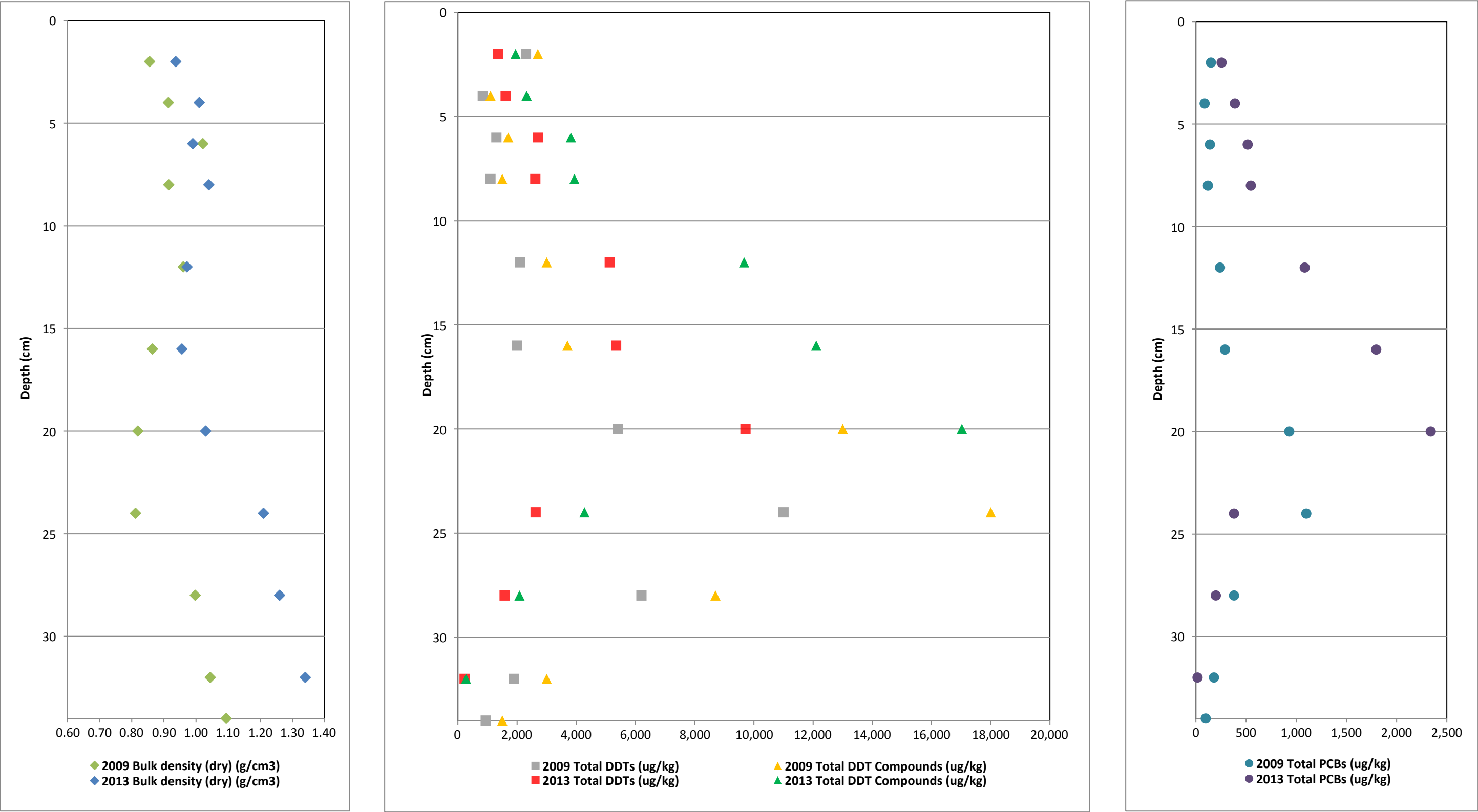
Figure 29. Vertical Profiles of Bulk Density and COCs for Core BA9BC First MNR Report Palos Verdes Shelf (OU 5 of the Montrose Chemical Corp. Superfund Site) Los Angeles County, California
