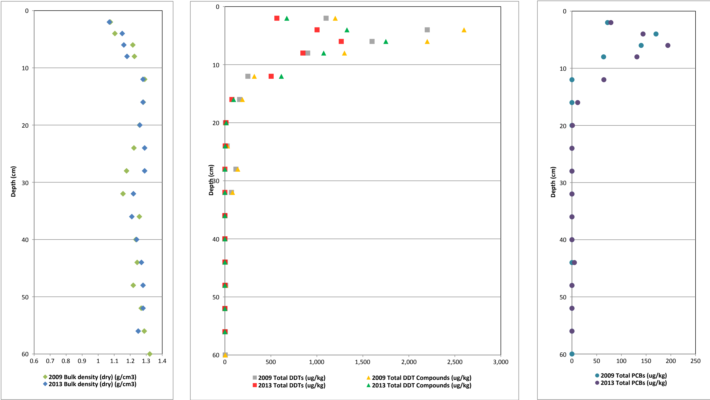
Figure 1. Vertical Profiles of Bulk Density, Total DDTs, and Total DDT Compounds for Core BA1B First MNR Report Palos Verdes Shelf (OU 5 of the Montrose Chemical Corp. Superfund Site) Los Angeles County, California
