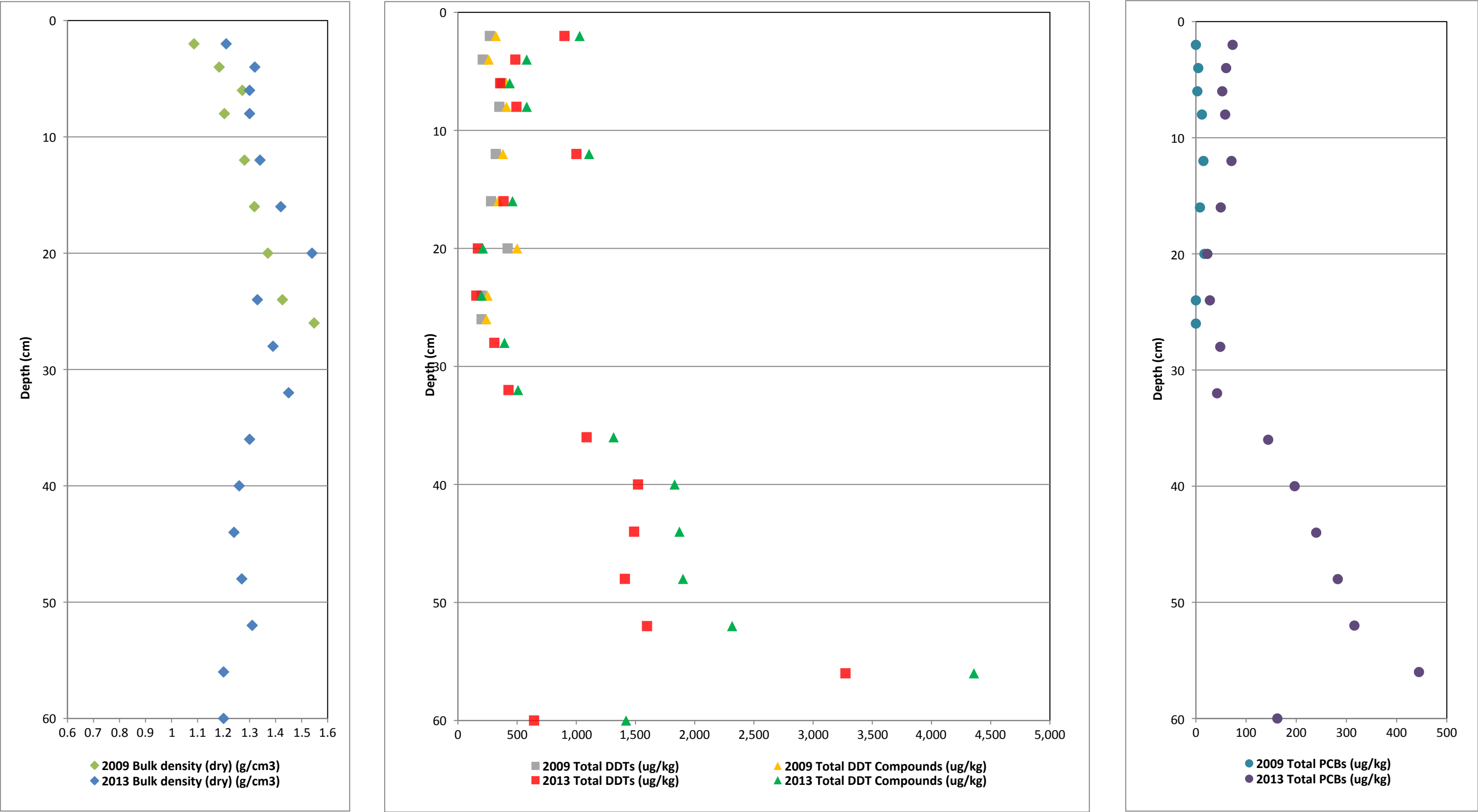
Figure 23. Vertical Profiles of Bulk Density and COCs for Core BA7DC First MNR Report Palos Verdes Shelf (OU 5 of the Montrose Chemical Corp. Superfund Site) Los Angeles County, California
