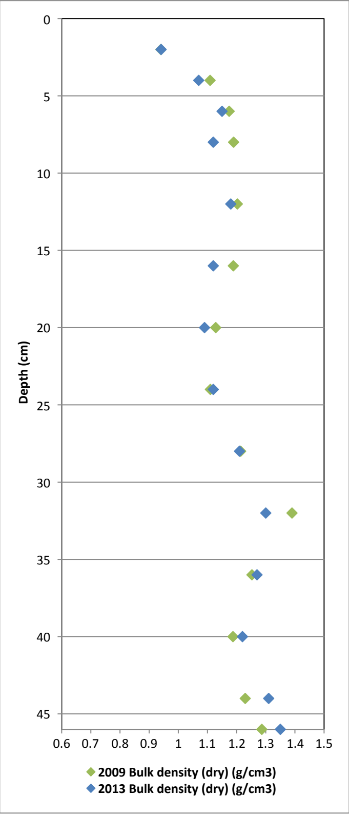
Figure 2. Vertical Profiles of Bulk Density and COCs for Core BA1C First MNR Report Palos Verdes Shelf (OU 5 of the Montrose Chemical Corp. Superfund Site) Los Angeles County, California
