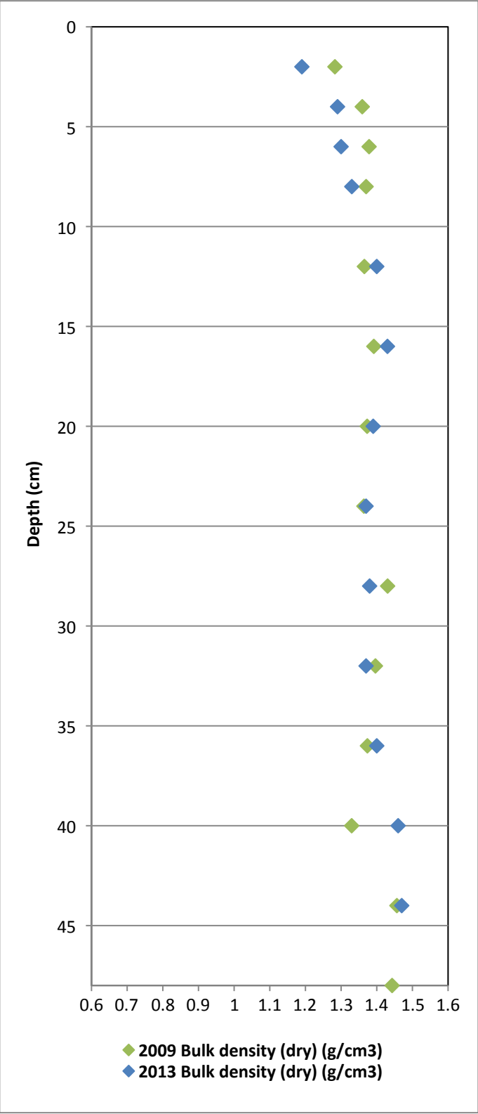
Figure 6. Vertical Profiles of Bulk Density and COCs for Core BA2DC First MNR Report Palos Verdes Shelf (OU 5 of the Montrose Chemical Corp. Superfund Site) Los Angeles County, California
