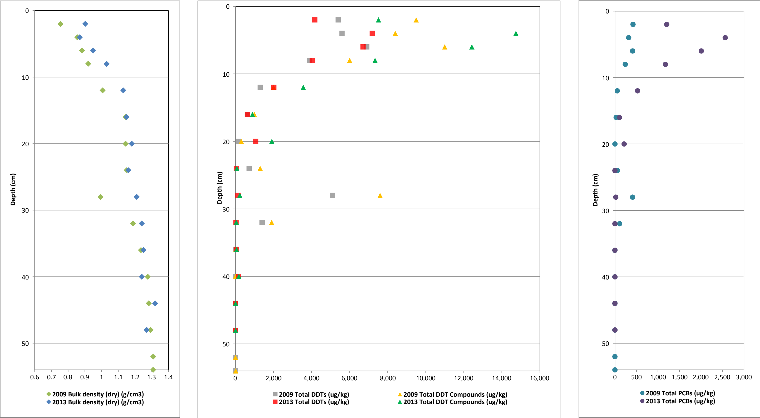
Figure 20. Vertical Profiles of Bulk Density and COCs for Core BA7B First MNR Report Palos Verdes Shelf (OU 5 of the Montrose Chemical Corp. Superfund Site) Los Angeles County, California
