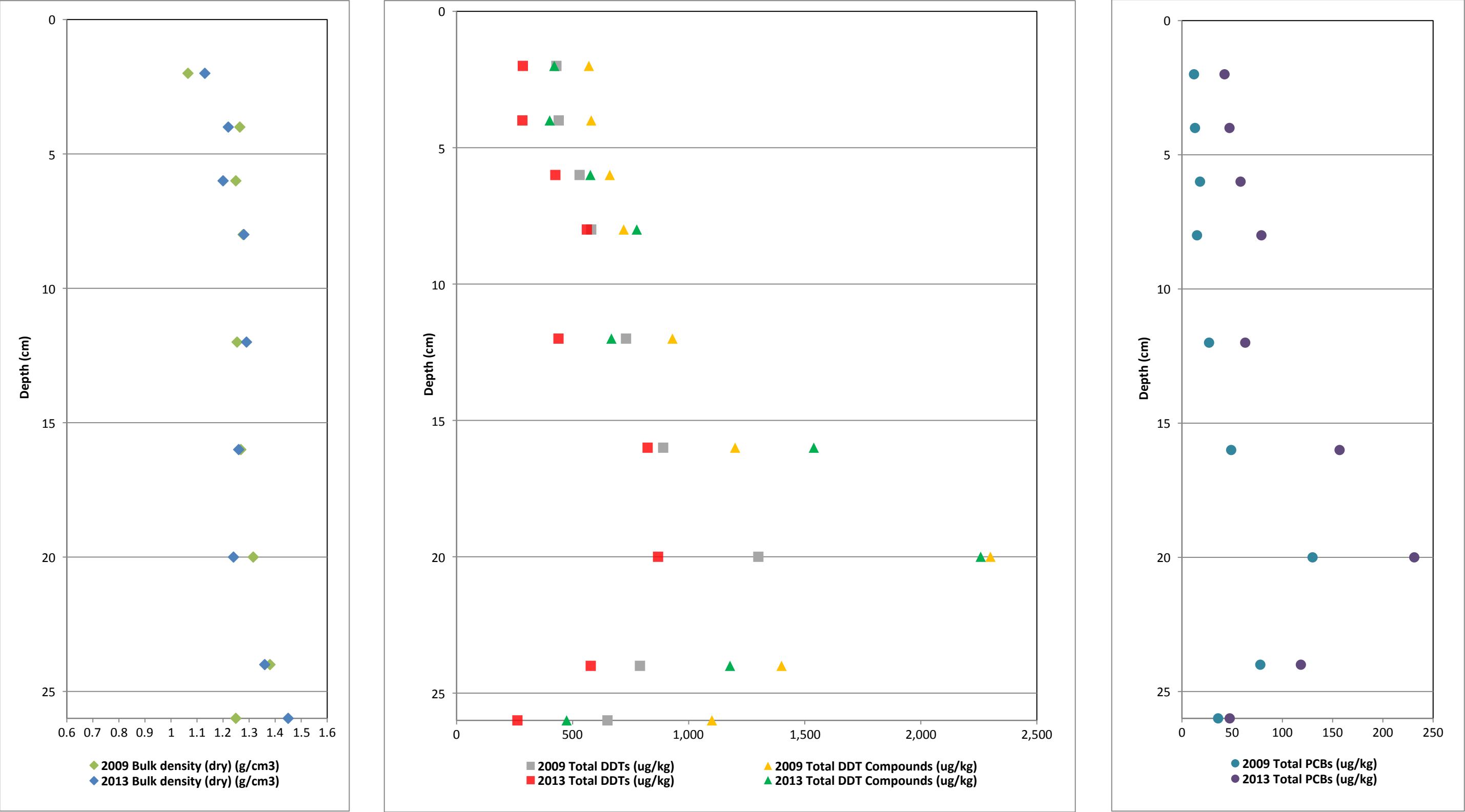
Figure 3. Vertical Profiles of Bulk Density and COCs for Core BA1DC First MNR Report Palos Verdes Shelf (OU 5 of the Montrose Chemical Corp. Superfund Site) Los Angeles County, California
