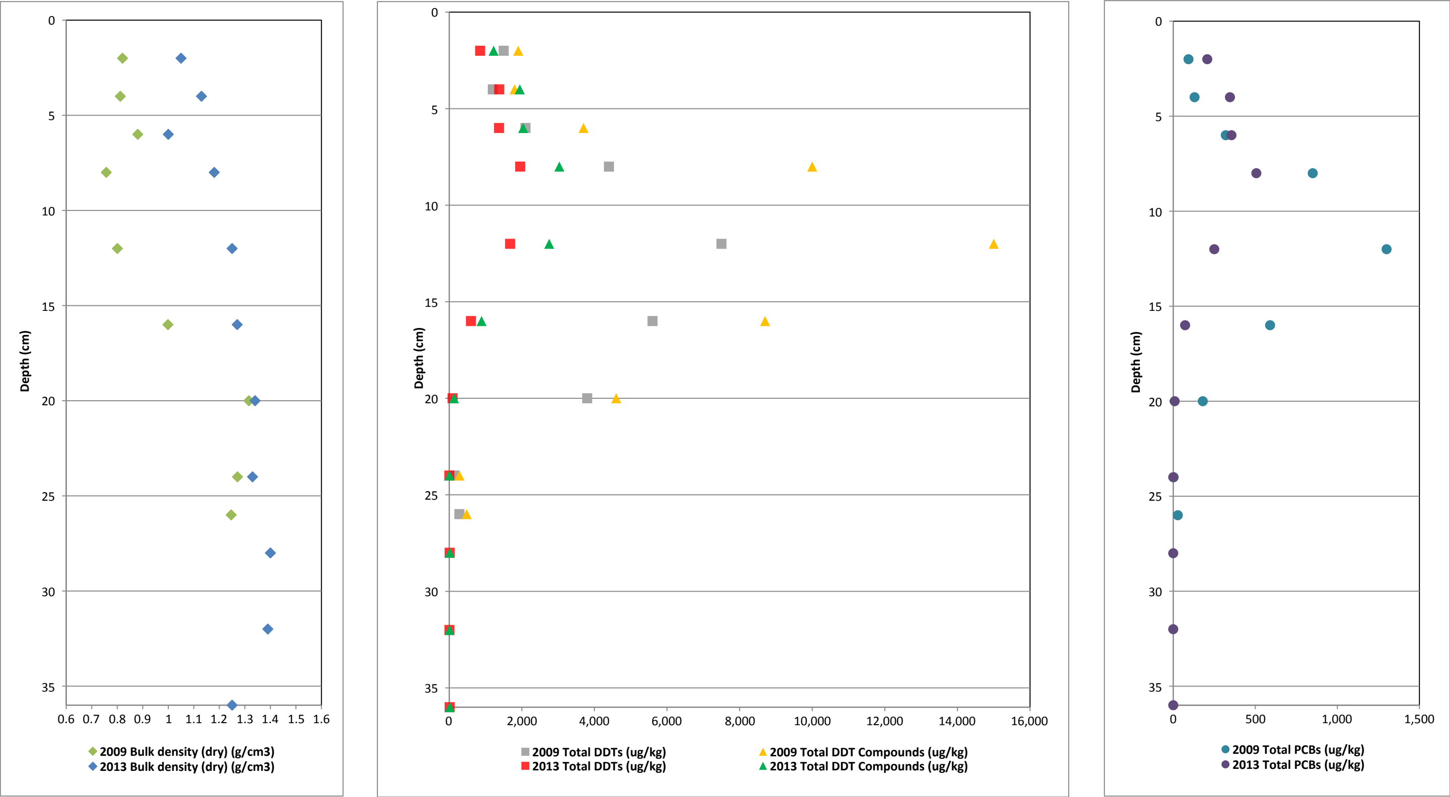
Figure 25. Vertical Profiles of Bulk Density and COCs for Core BA8BC First MNR Report Palos Verdes Shelf (OU 5 of the Montrose Chemical Corp. Superfund Site) Los Angeles County, California
