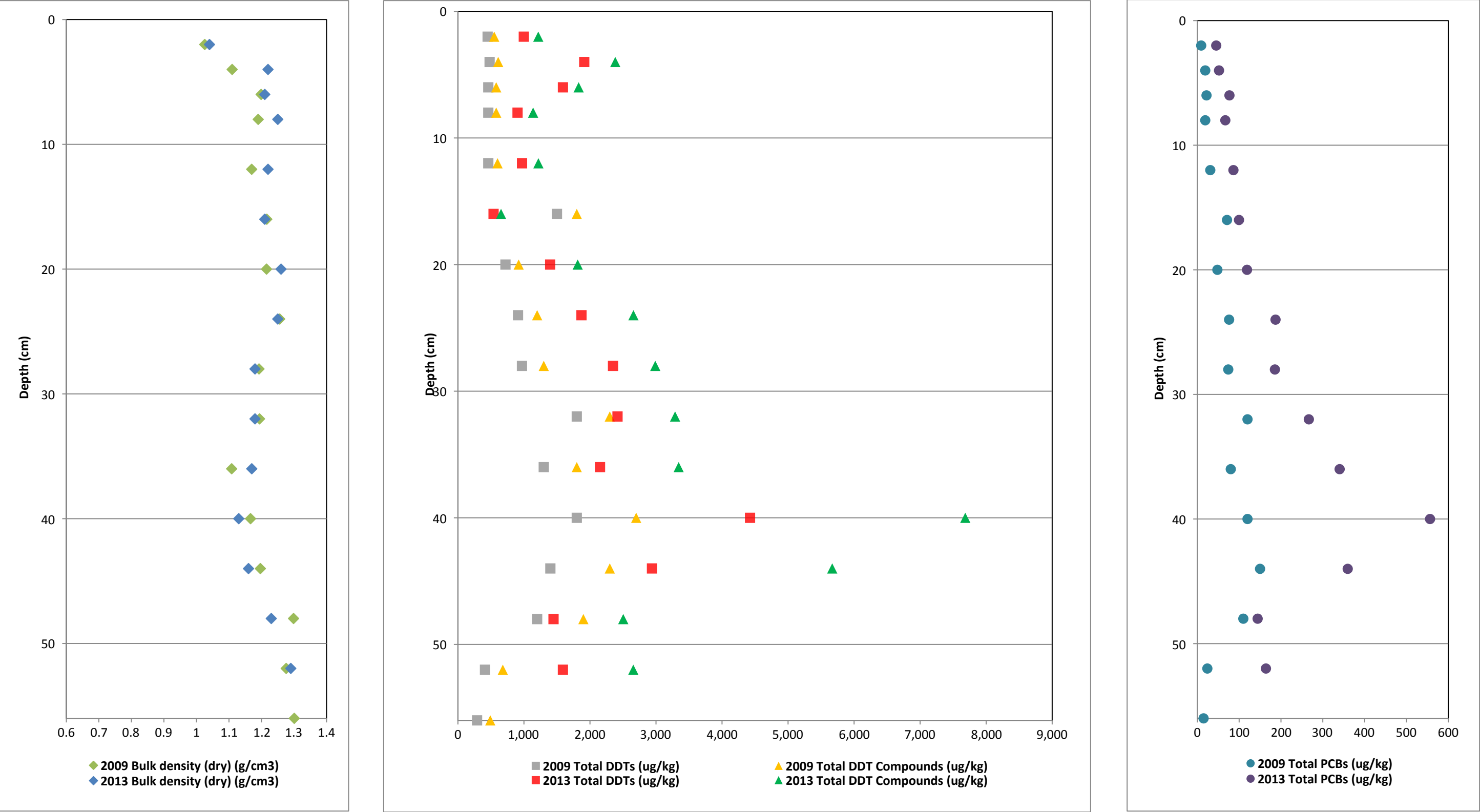
Figure 19. Vertical Profiles of Bulk Density and COCs for Core BA6DC First MNR Report Palos Verdes Shelf (OU 5 of the Montrose Chemical Corp. Superfund Site) Los Angeles County, California
