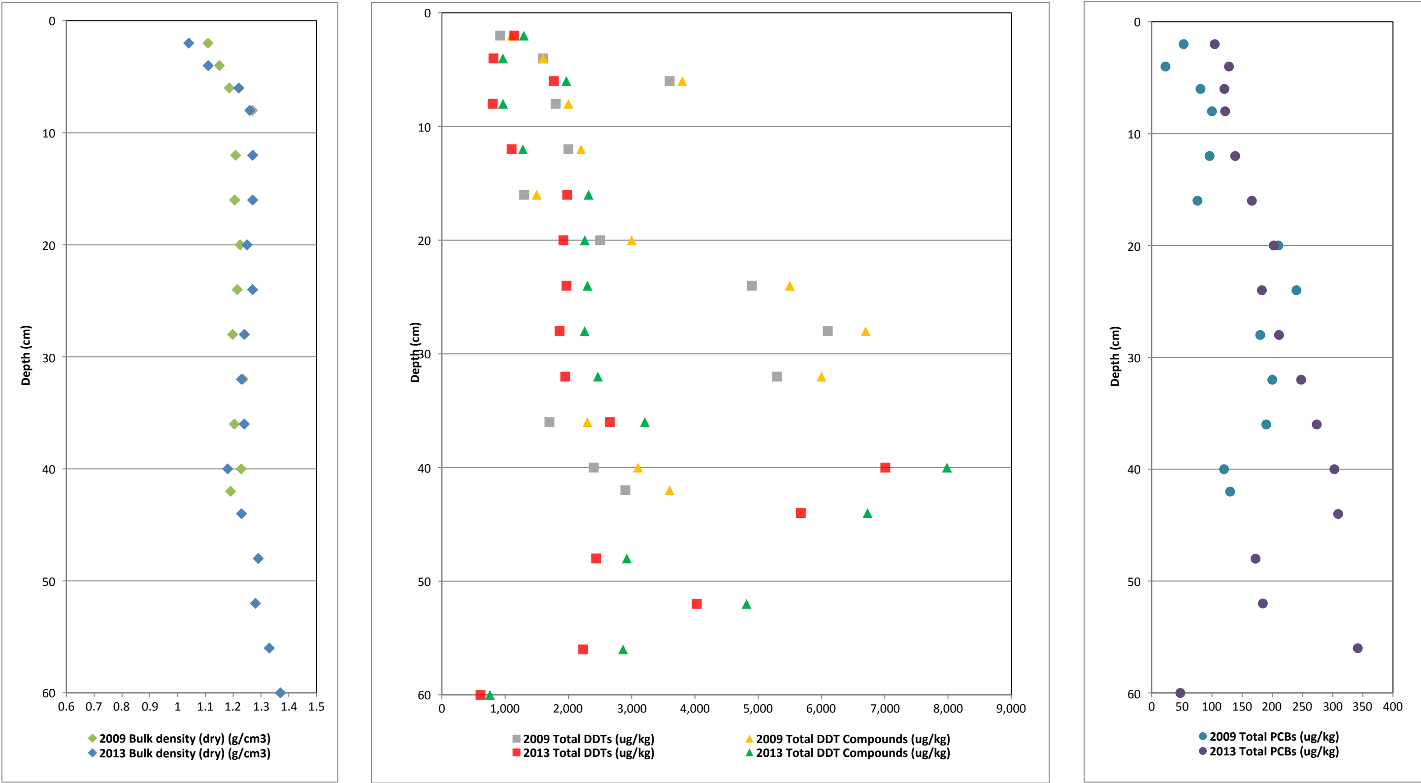
Figure 27. Vertical Profiles of Bulk Density and COCs for Core BA8DC First MNR Report Palos Verdes Shelf (OU 5 of the Montrose Chemical Corp. Superfund Site) Los Angeles County, California
