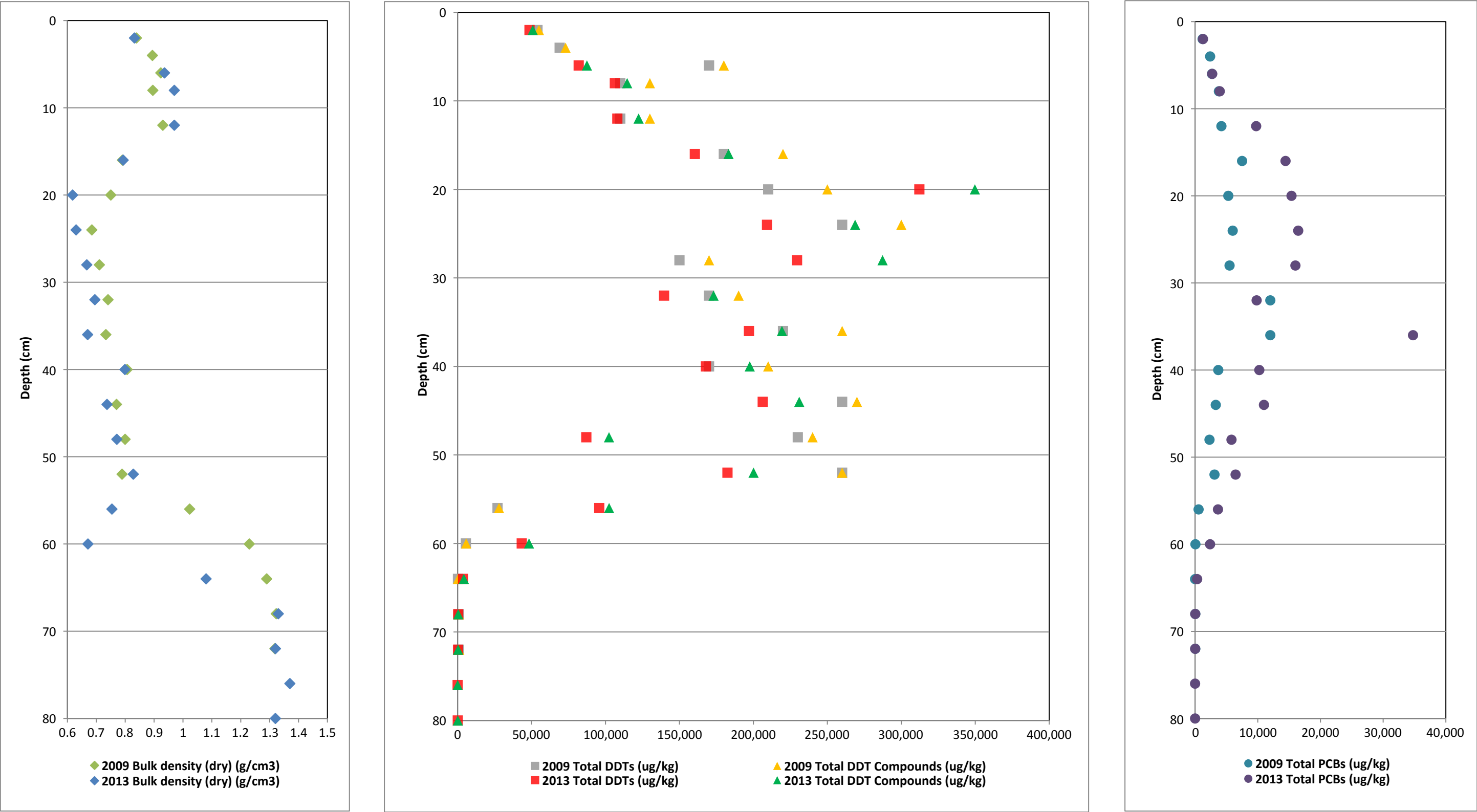
Figure 26. Vertical Profiles of Bulk Density and COCs for Core BA8C First MNR Report Palos Verdes Shelf (OU 5 of the Montrose Chemical Corp. Superfund Site) Los Angeles County, California
