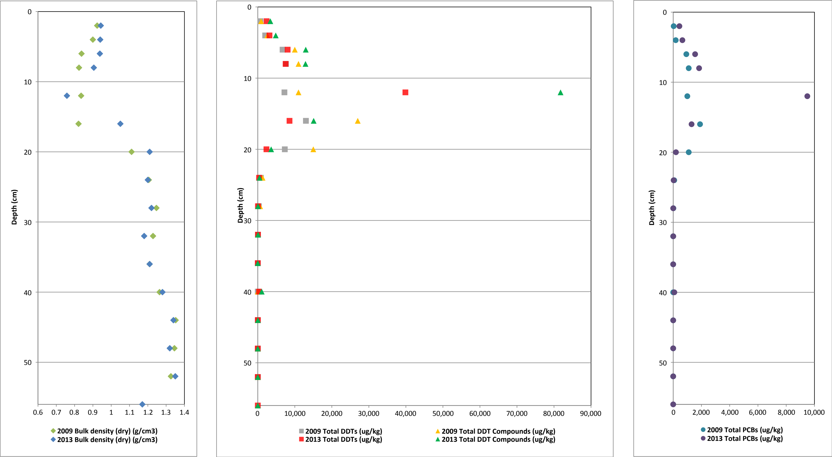
Figure 10. Vertical Profiles of Bulk Density and COCs for Core BA4B First MNR Report Palos Verdes Shelf (OU 5 of the Montrose Chemical Corp. Superfund Site) Los Angeles County, California
