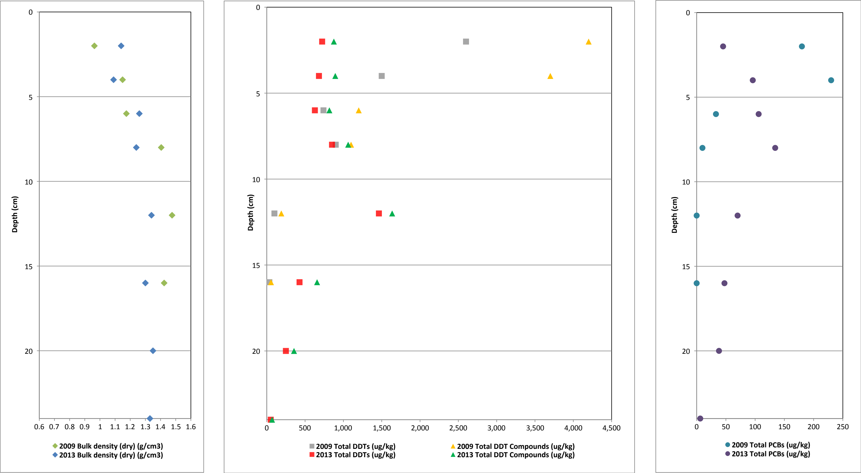
Figure 21. Vertical Profiles of Bulk Density and COCs for Core BA7BC First MNR Report Palos Verdes Shelf (OU 5 of the Montrose Chemical Corp. Superfund Site) Los Angeles County, California
