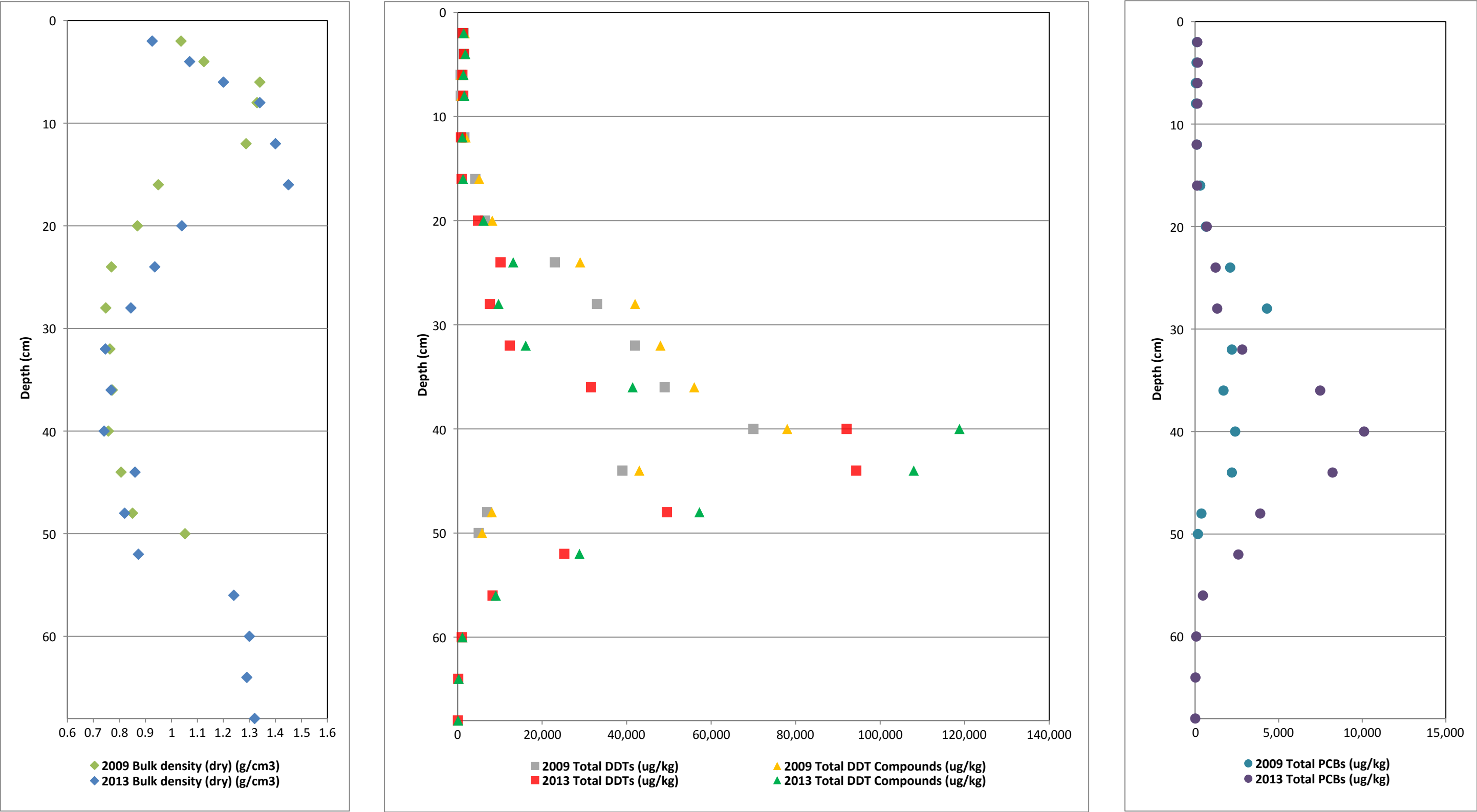
Figure 22. Vertical Profiles of Bulk Density and COCs for Core BA7C First MNR Report Palos Verdes Shelf (OU 5 of the Montrose Chemical Corp. Superfund Site) Los Angeles County, California
