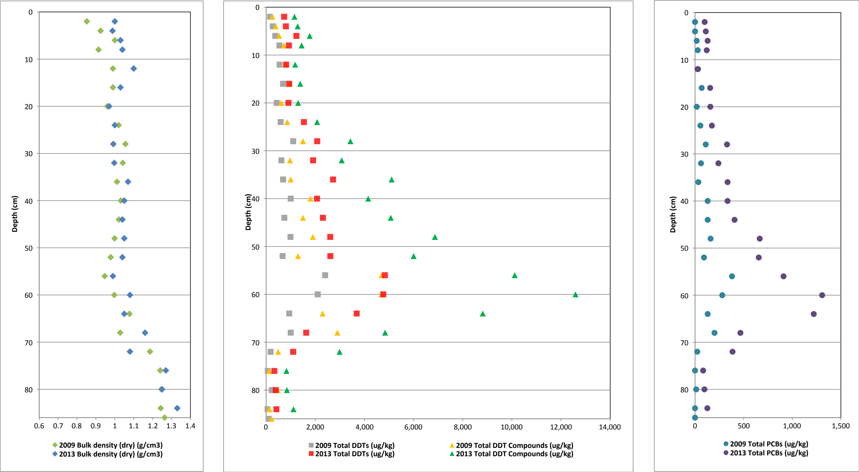
Figure 12. Vertical Profiles of Bulk Density and COCs for Core BA4DC First MNR Report Palos Verdes Shelf (OU 5 of the Montrose Chemical Corp. Superfund Site) Los Angeles County, California
