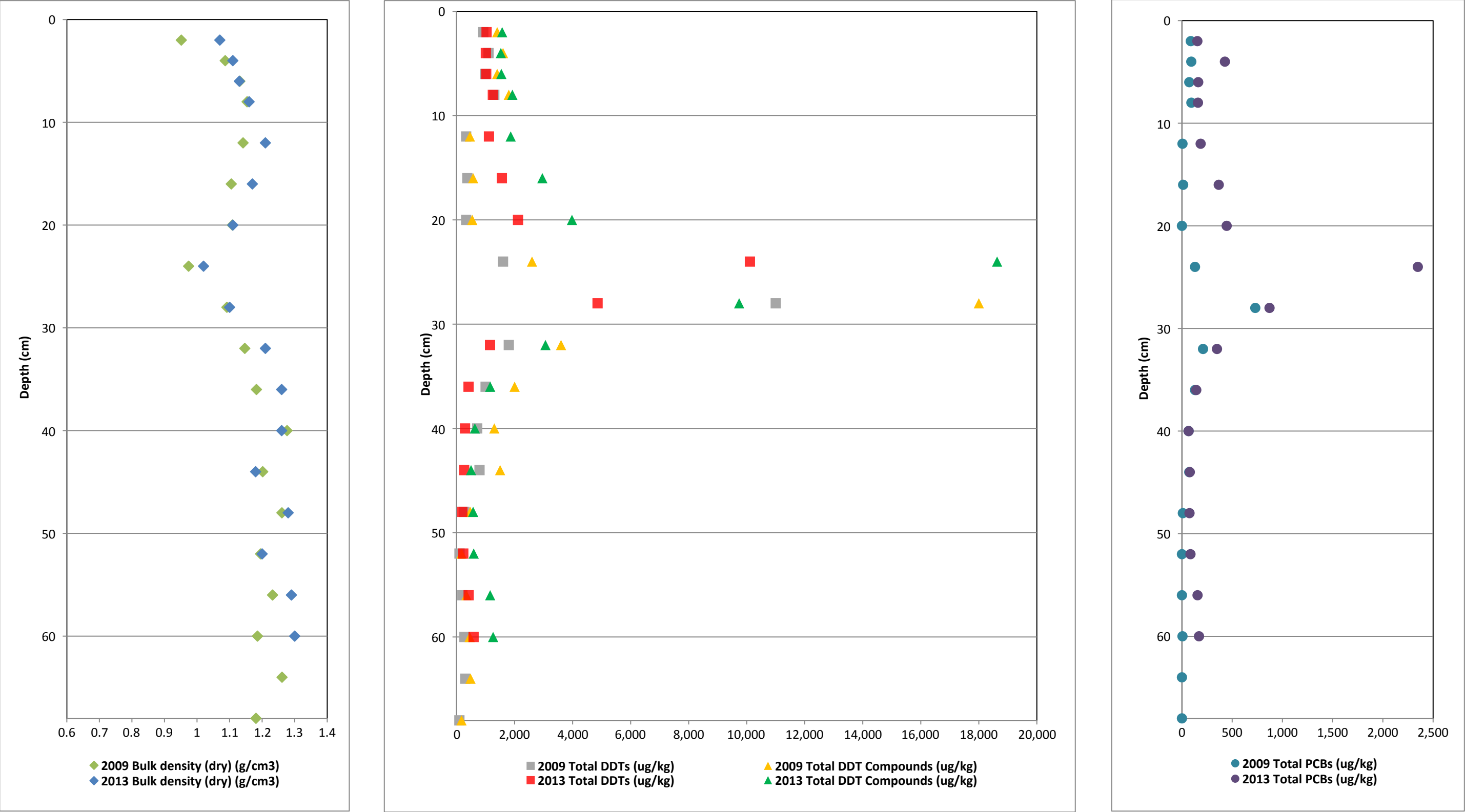
Figure 5. Vertical Profiles of Bulk Density and COCs for Core BA2C First MNR Report Palos Verdes Shelf (OU 5 of the Montrose Chemical Corp. Superfund Site) Los Angeles County, California
