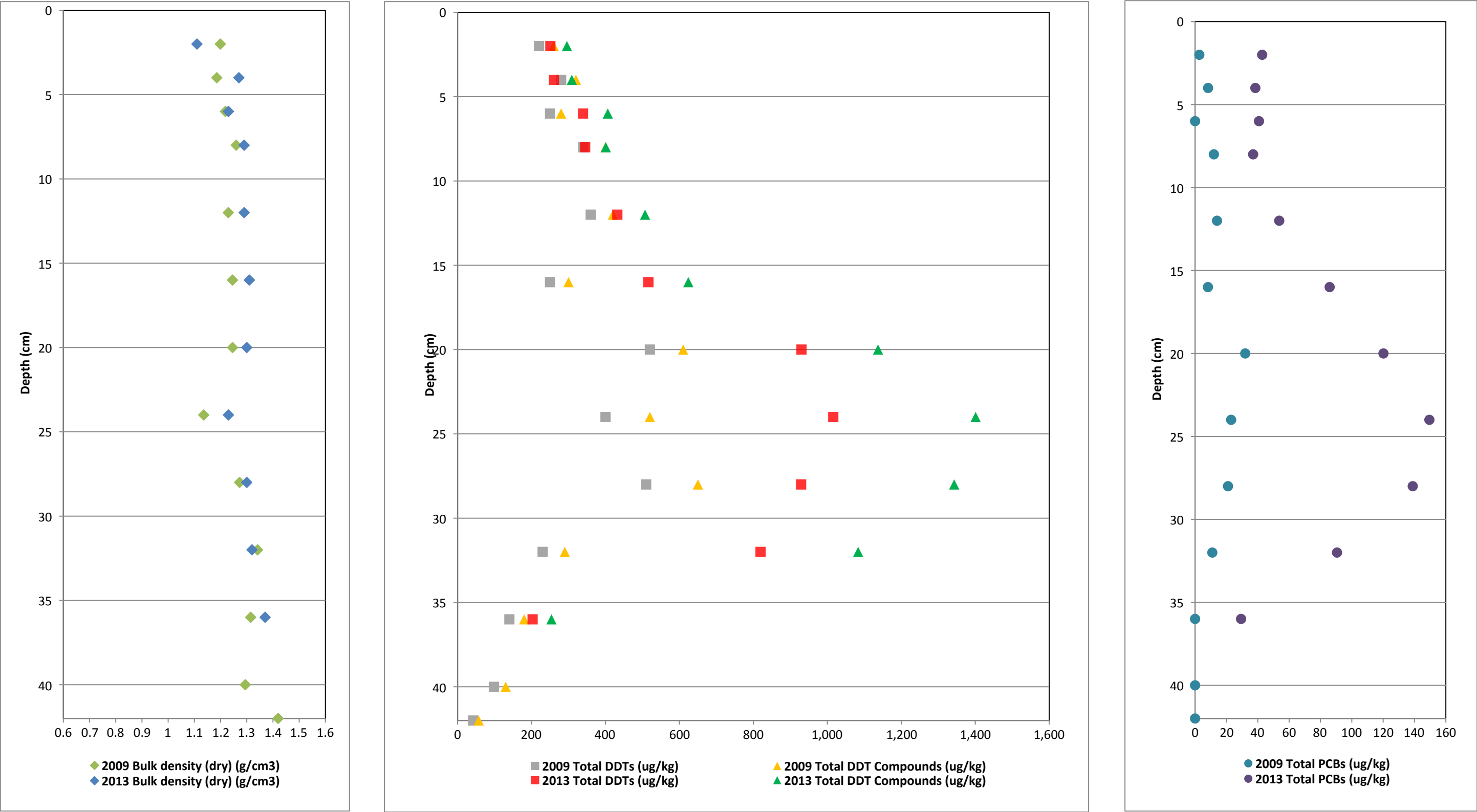
Figure 34. Vertical Profiles of Bulk Density and COCs for Core BA10DC First MNR Report Palos Verdes Shelf (OU 5 of the Montrose Chemical Corp. Superfund Site) Los Angeles County, California
