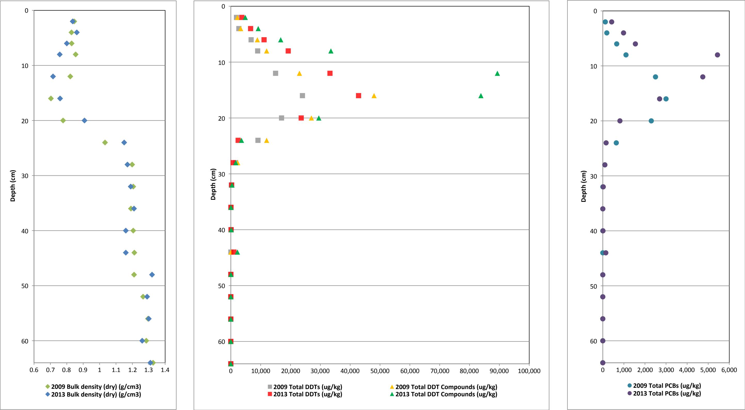
Figure 13. Vertical Profiles of Bulk Density and COCs for Core BA5B First MNR Report Palos Verdes Shelf (OU 5 of the Montrose Chemical Corp. Superfund Site) Los Angeles County, California
