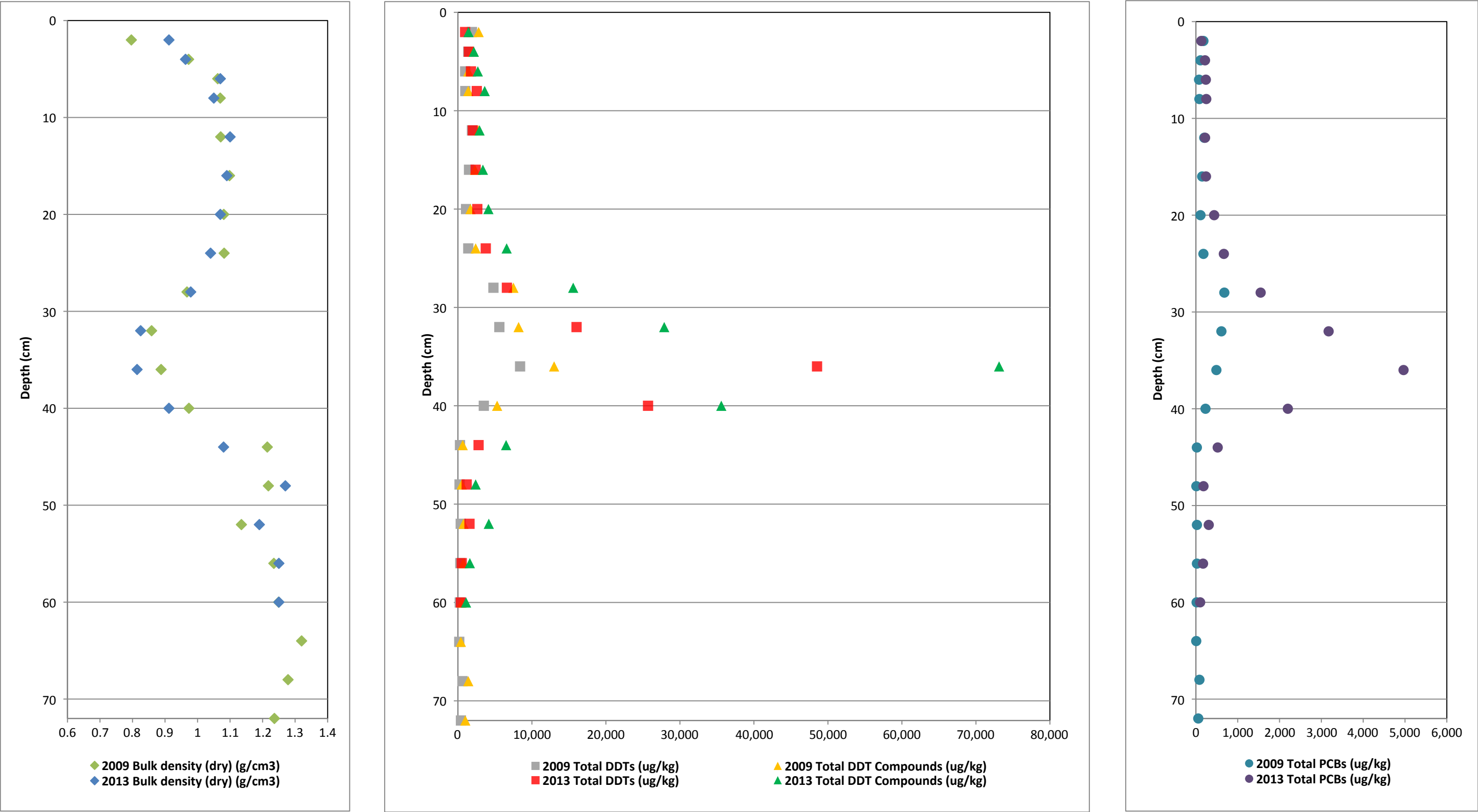
Figure 11. Vertical Profiles of Bulk Density and COCs for Core BA4C First MNR Report Palos Verdes Shelf (OU 5 of the Montrose Chemical Corp. Superfund Site) Los Angeles County, California
