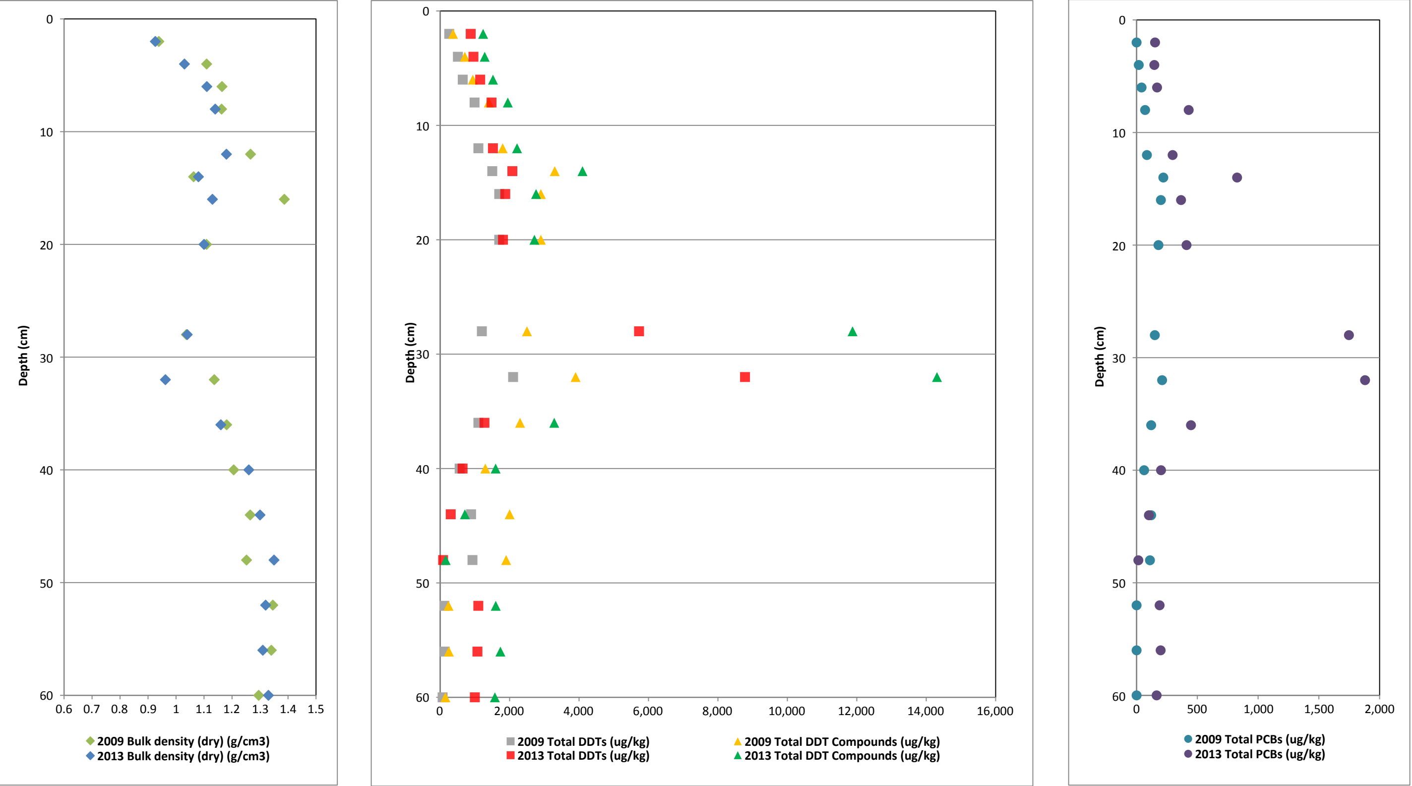
Figure 8. Vertical Profiles of Bulk Density and COCs for Core BA3C First MNR Report Palos Verdes Shelf (OU 5 of the Montrose Chemical Corp. Superfund Site) Los Angeles County, California
