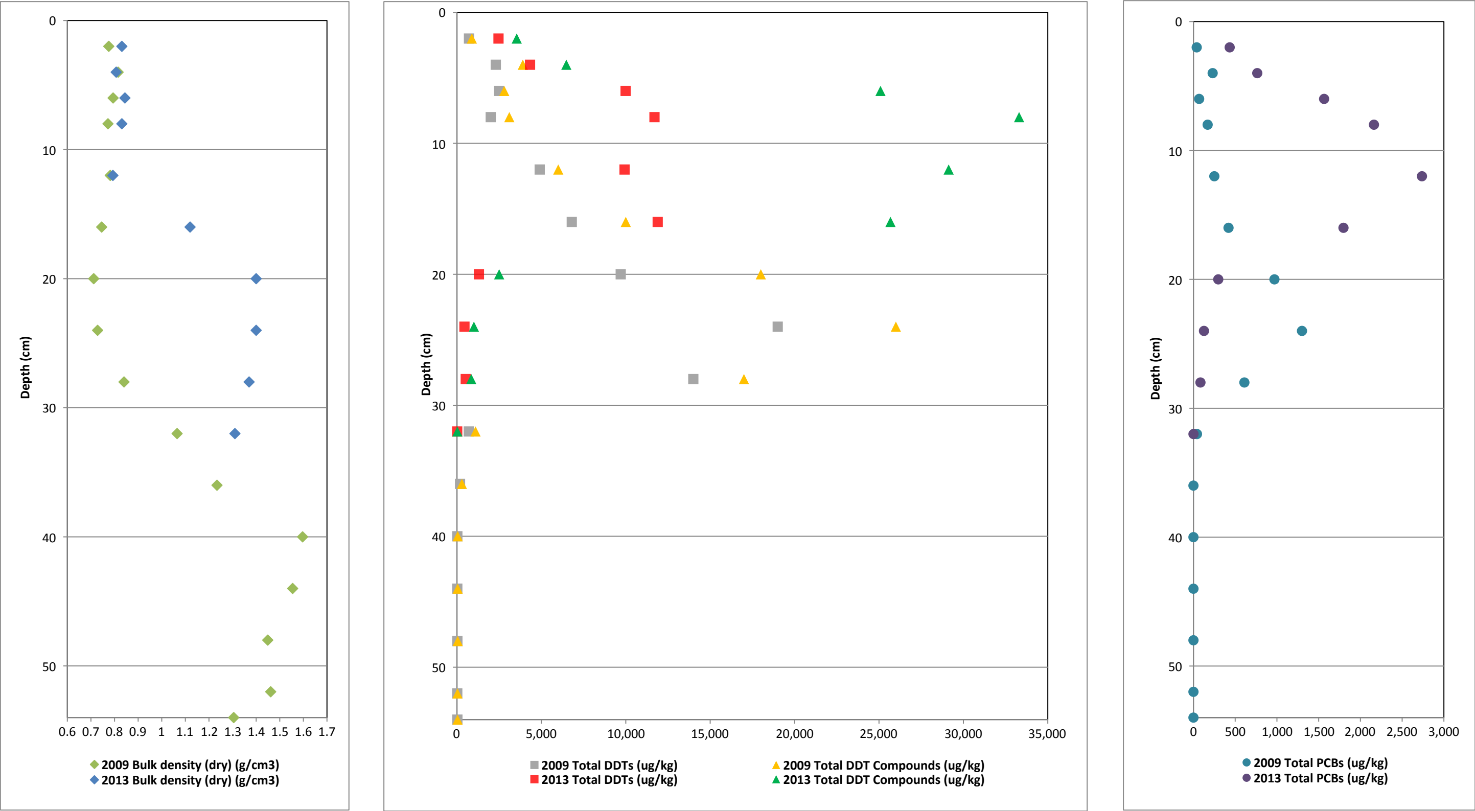
Figure 17. Vertical Profiles of Bulk Density and COCs for Core BA6BC First MNR Report Palos Verdes Shelf (OU 5 of the Montrose Chemical Corp. Superfund Site) Los Angeles County, California
