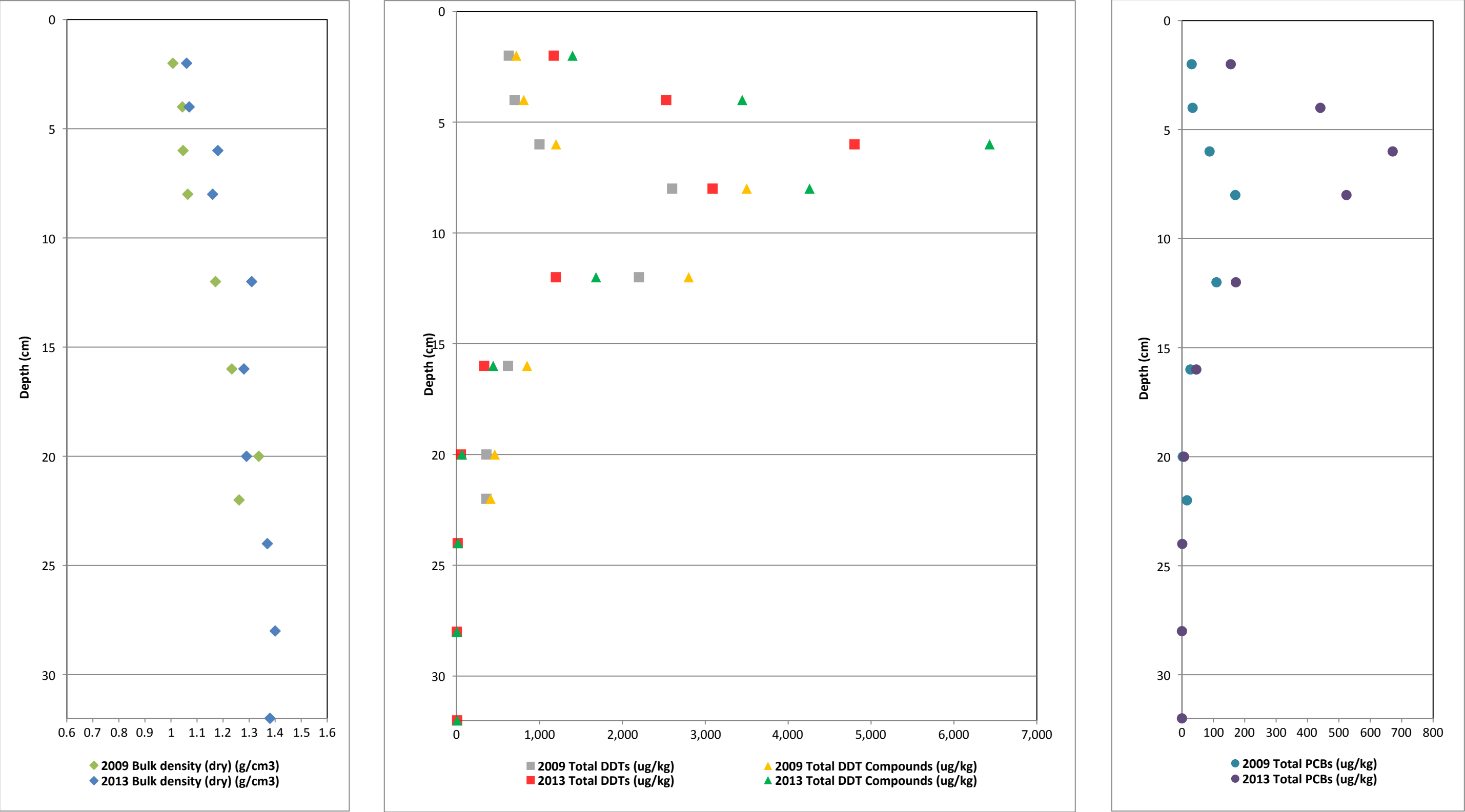
Figure 7. Vertical Profiles of Bulk Density and COCs for Core BA3B First MNR Report Palos Verdes Shelf (OU 5 of the Montrose Chemical Corp. Superfund Site) Los Angeles County, California
