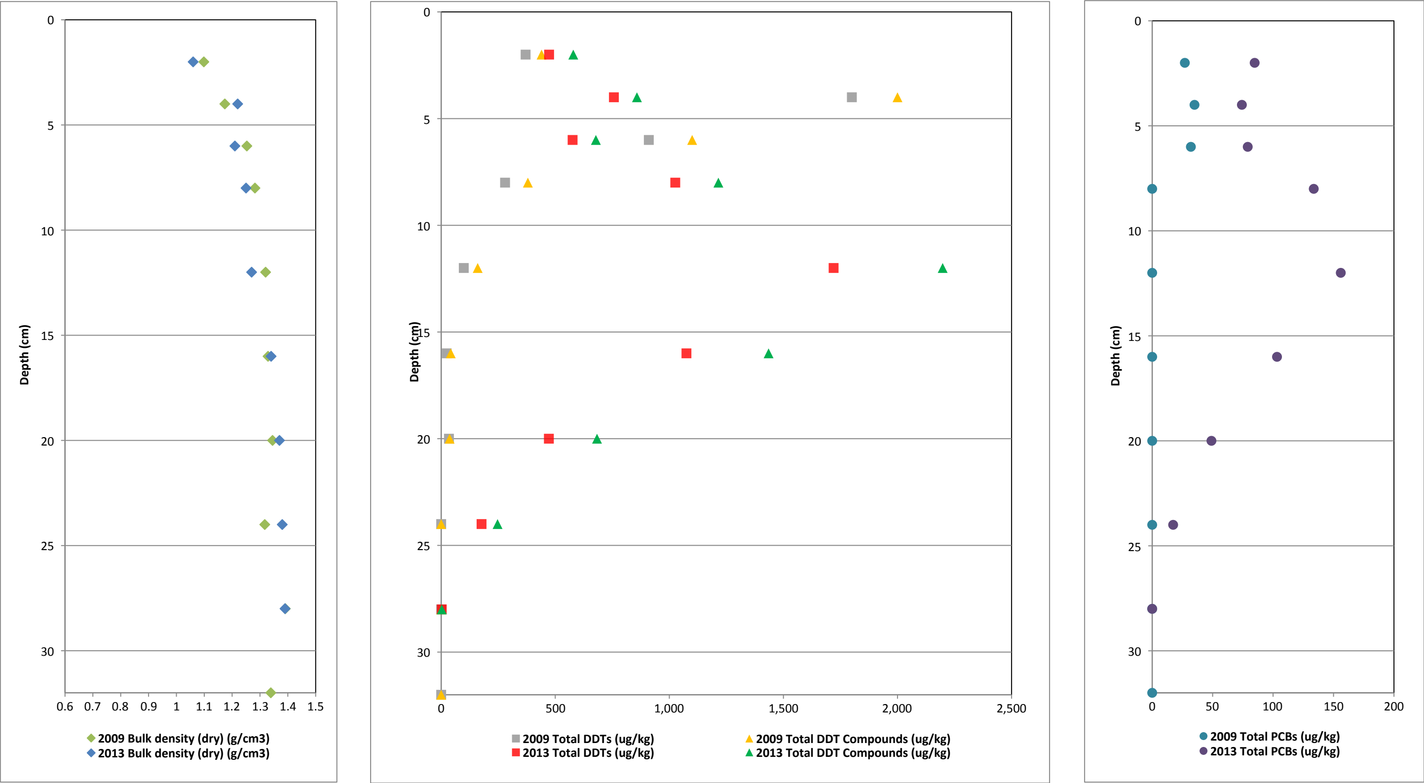
Figure 32. Vertical Profiles of Bulk Density and COCs for Core BA10B First MNR Report Palos Verdes Shelf (OU 5 of the Montrose Chemical Corp. Superfund Site) Los Angeles County, California
