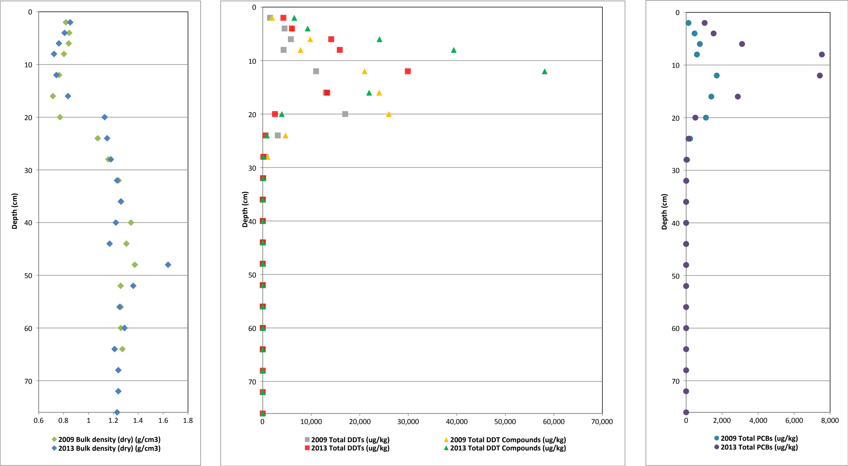
Figure 16. Vertical Profiles of Bulk Density and COCs for Core BA6B First MNR Report Palos Verdes Shelf (OU 5 of the Montrose Chemical Corp. Superfund Site) Los Angeles County, California
