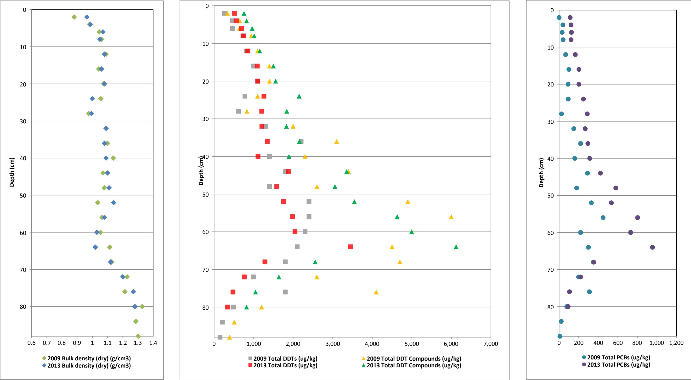
Figure 15. Vertical Profiles of Bulk Density and COCs for Core BA5DC First MNR Report Palos Verdes Shelf (OU 5 of the Montrose Chemical Corp. Superfund Site) Los Angeles County, California
