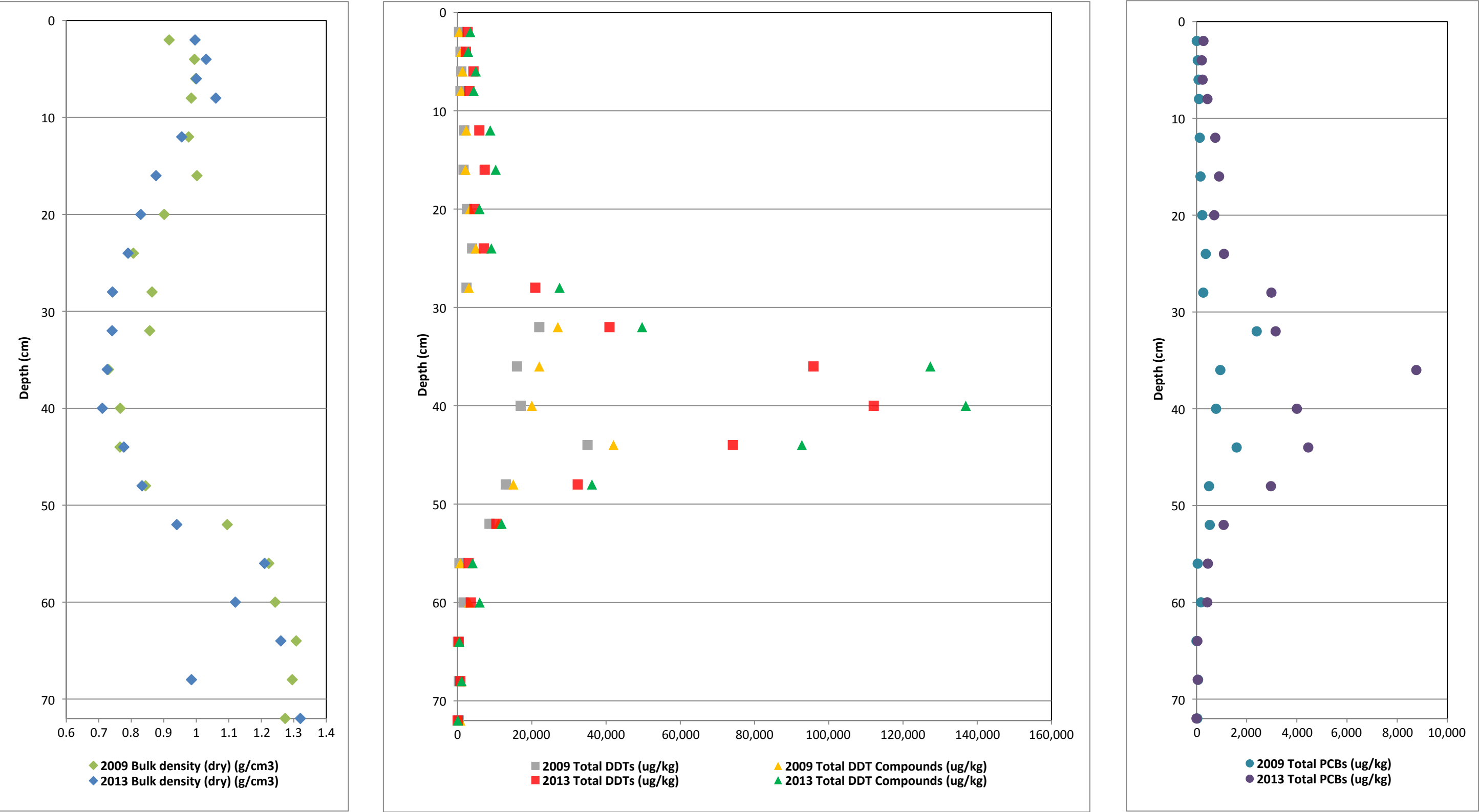
Figure 18. Vertical Profiles of Bulk Density and COCs for Core BA6C First MNR Report Palos Verdes Shelf (OU 5 of the Montrose Chemical Corp. Superfund Site) Los Angeles County, California
