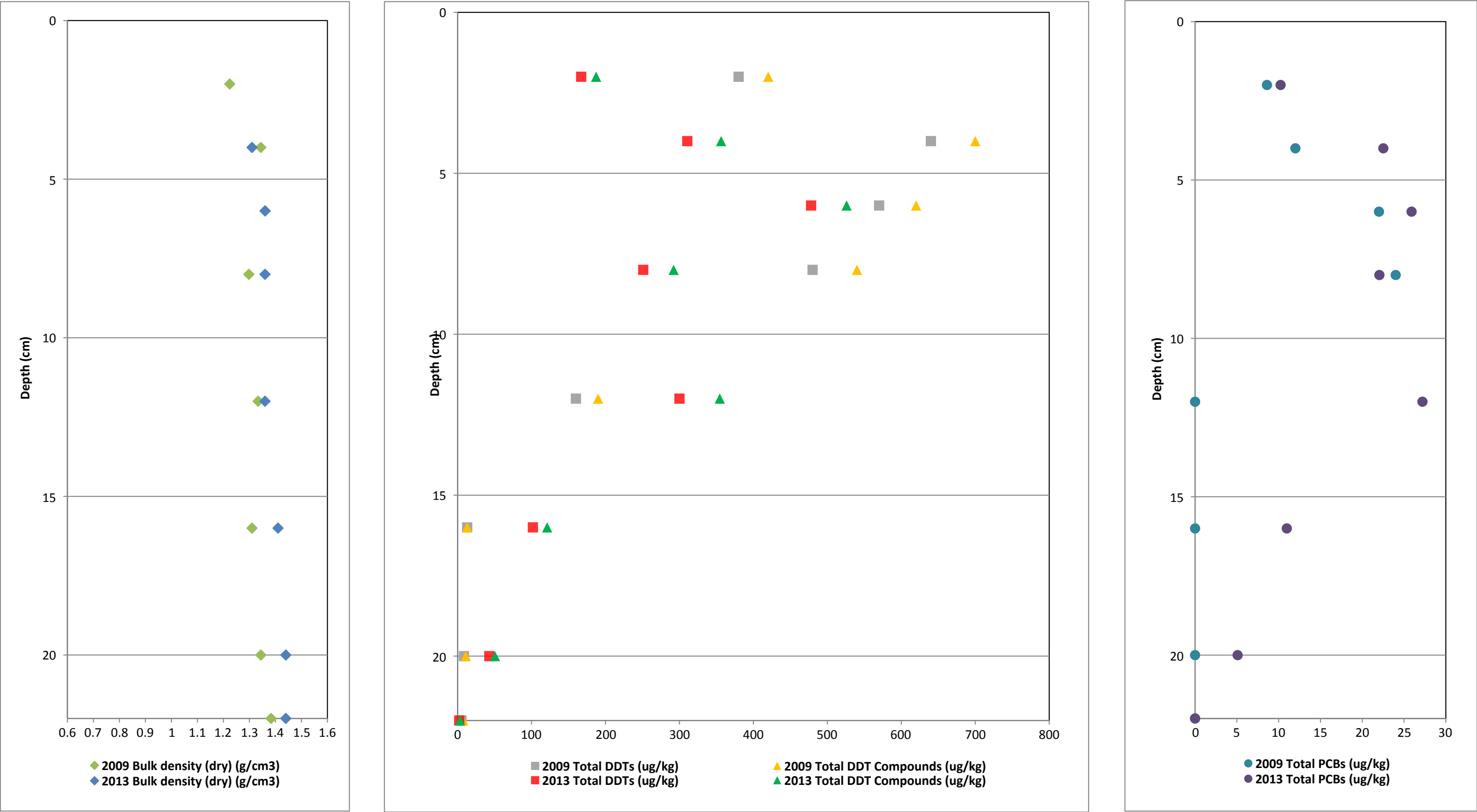
Figure 33. Vertical Profiles of Bulk Density and COCs for Core BA10C First MNR Report Palos Verdes Shelf (OU 5 of the Montrose Chemical Corp. Superfund Site) Los Angeles County, California
