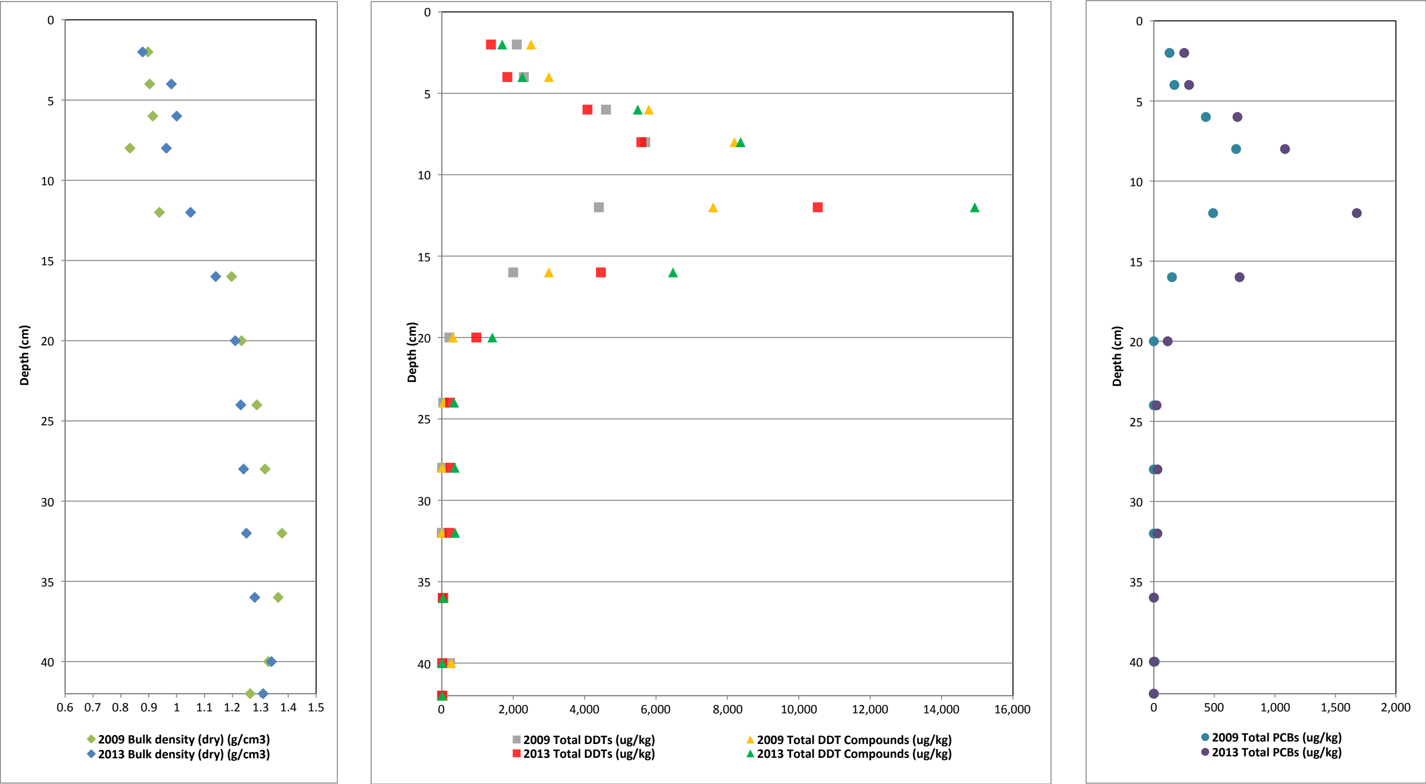
Figure 28. Vertical Profiles of Bulk Density and COCs for Core BA9B First MNR Report Palos Verdes Shelf (OU 5 of the Montrose Chemical Corp. Superfund Site) Los Angeles County, California
