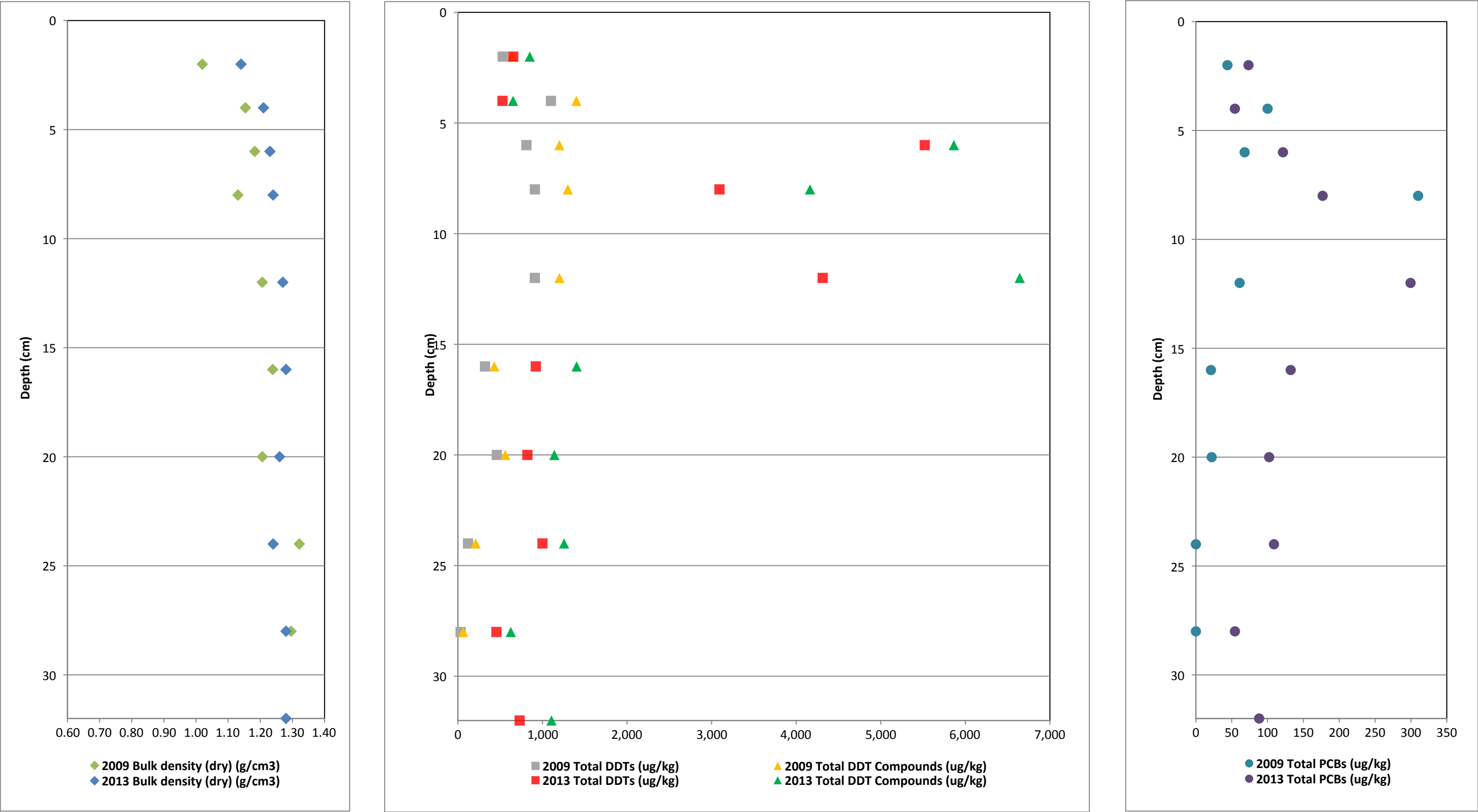
Figure 30. Vertical Profiles of Bulk Density and COCs for Core BA9C First MNR Report Palos Verdes Shelf (OU 5 of the Montrose Chemical Corp. Superfund Site) Los Angeles County, California
