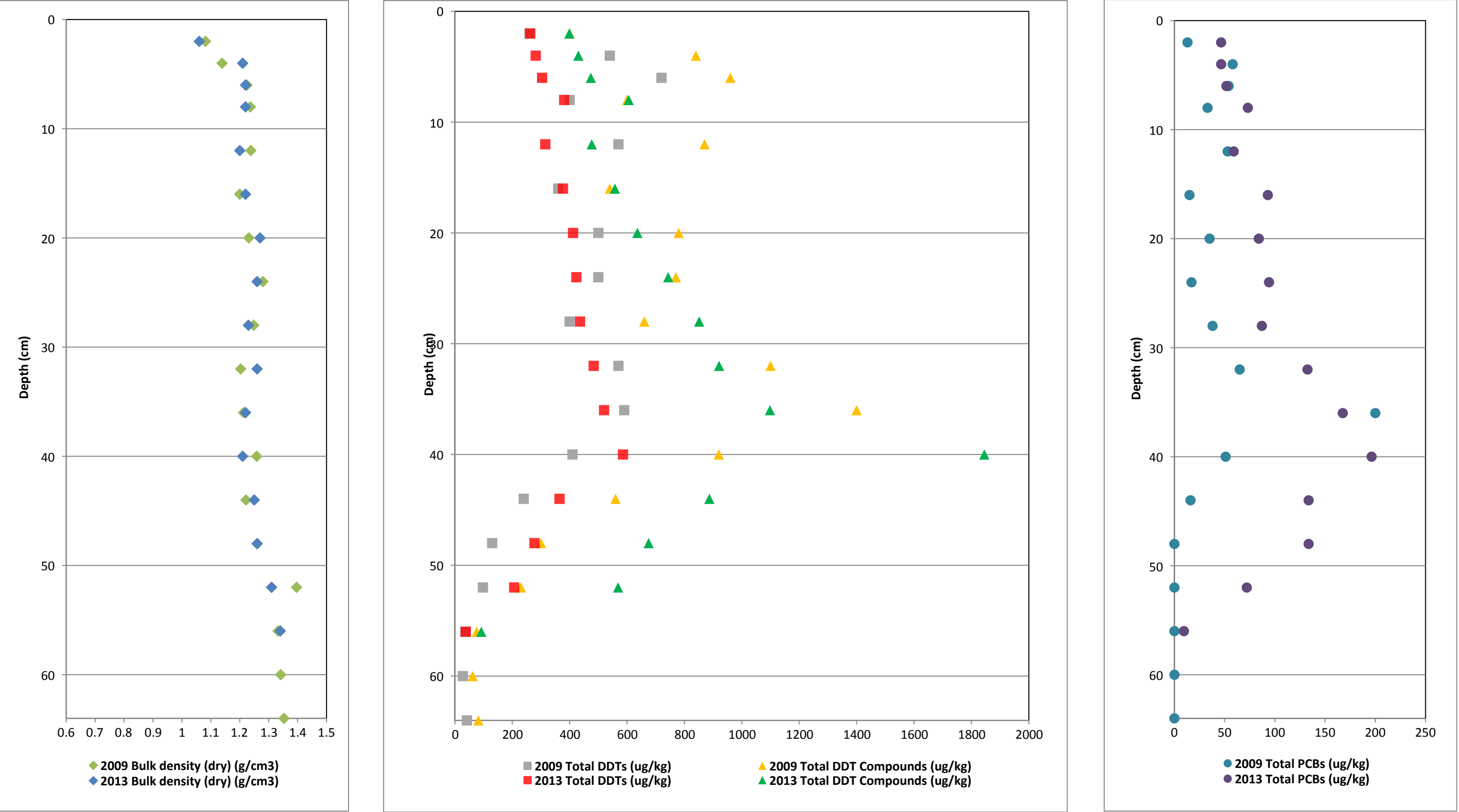
Figure 9. Vertical Profiles of Bulk Density and COCs for Core BA3DC First MNR Report Palos Verdes Shelf (OU 5 of the Montrose Chemical Corp. Superfund Site) Los Angeles County, California
